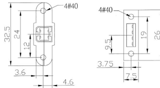
Screw Lock Cable Connectors
